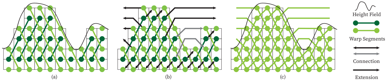
Fig. 12. A Variant of Through-thickness Structure: (a) A height field is discretized in to grids. Two sets of diagonal segments are generated to connect the circles. (b) First, the light green circles on the surface are connected to the dark green circles next to them (black double arrows). Then, the free ends of segments in the concave part of the height field are paired and connected (gray double arrow). Finally, the rest of the free ends are extended to the two sides of the slice (black single arrow). (c) The connected and extended segments form the paths for the warp yarns. The part above the height field surface will be trimmed in post-process.
