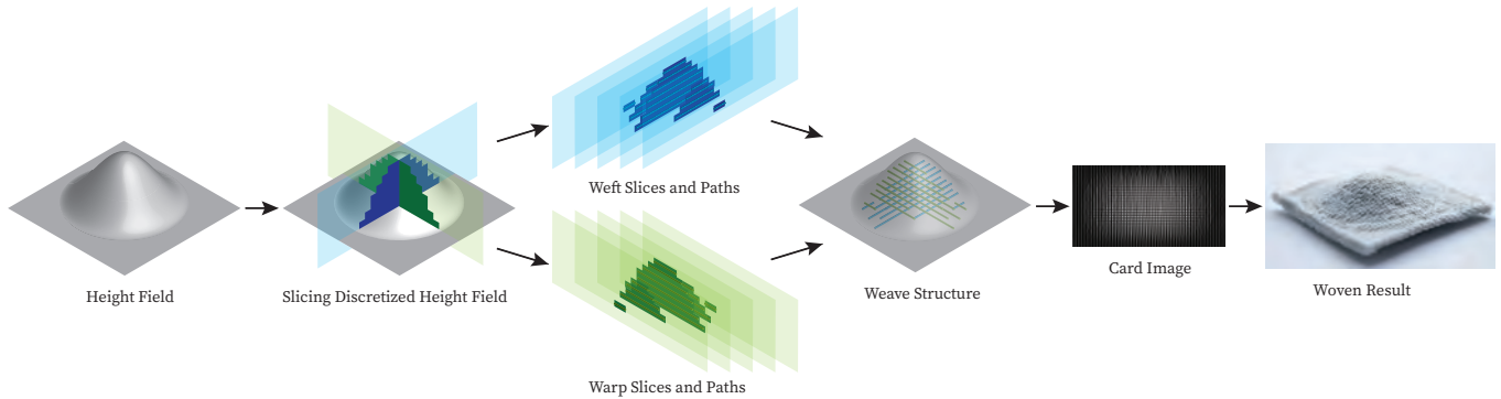
Fig. 6. The Pipeline of Our Method
