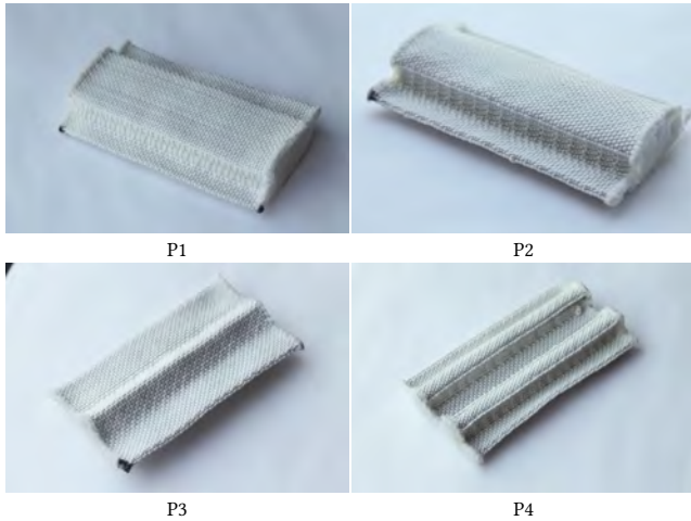
Fig. 14. Warp Extrusion Samples: P1 and P2 are generated from the same height field. The loose yarns in P1 are moved inside the fabric in P2, creating a neat pattern and sharp cliff on the selvedge face. P3 shows a triangular bump. P4 shows double square bumps.
