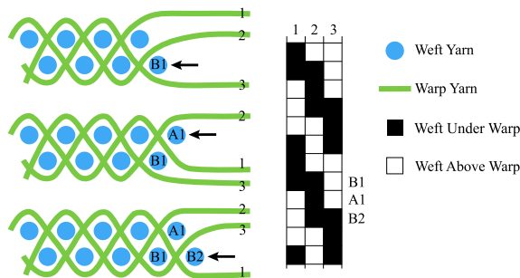
Fig. 2. By arranging the raised and lowered warp ends properly, weft yarns can be inserted to form a multi-layer structure. The card image shows three columns of a 2-layer 3-twill fabric, where each row corresponds to a weft insertion and each column corresponds to a warp yarn. Left is a side view of the weaving sequence for three successive weft insertions, corresponding to the three labeled rows in the card image. Each weft is guided to the top or bottom layer by the card image.
