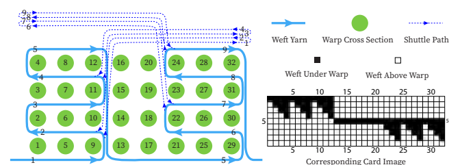
Fig. 8. Using weft turnarounds to create two separate rectangular bumps in weft slice. Each weft insertion corresponds to a row in the card image and each warp corresponds to a column, as indicated by the numbers.
