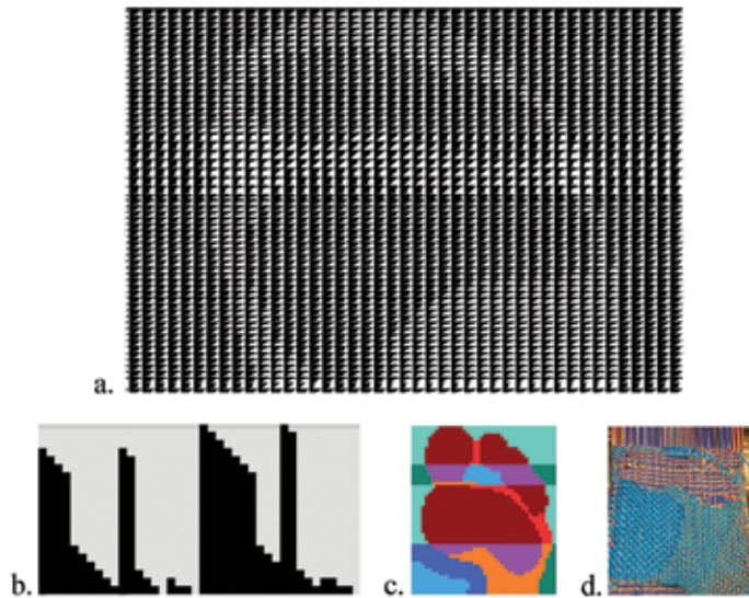
Fig. 5. Building depth in Pointcarre: a. card image for the toe, ball and arch of insole; b. use of supplementary wefts for depth in 2D Pointcarre file; c. graphic file for building layers; d. woven sample with thick and thin areas. (© VTRG 2018)
